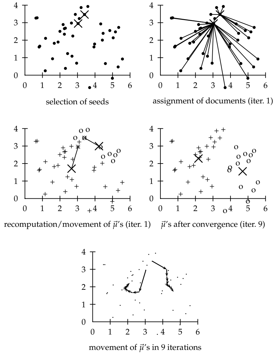
► Figure 16.6 A K -means example for K = 2 in \mathbb{R}^2 . The position of the two centroids ( \hat{\mu} 's shown as X 's in the top four panels) converges after nine iterations.
